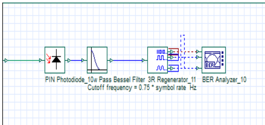
Fig. 7: Subsystem-3 (Receiver Section)
