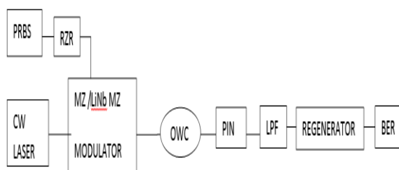
Fig. 1. Layout design of the inter-satellite communication system
