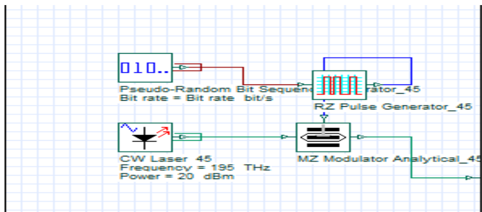
Fig. 5: Subsystem-1(Transmitter Section)
