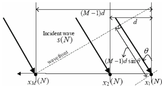
FIG. 4 UNIFORM LINEAR ARRAY OF M-ELEMENT
